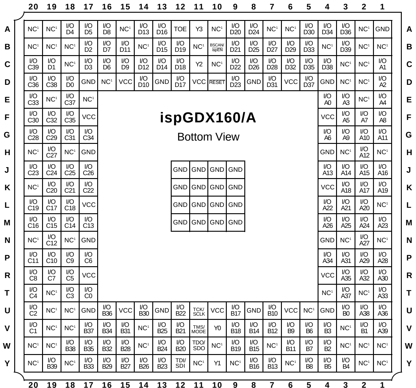
ispGDX160/A 272-Ball BGA Signal Diagram
