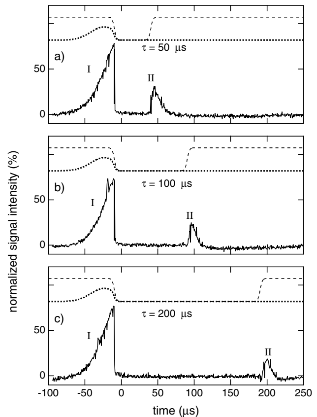
FIG. 2. Observed light pulse storage in a ^{87}\text{Rb} vapor cell. Examples are shown for storage times of (a) 50 \mu\text{s} , (b) 100 \mu\text{s} , and (c) 200 \mu\text{s} . (Background transmission from the control field, which leaks into the signal field detection optics, has been subtracted from these plots.) Signals are normalized to the peak intensity of the light transmitted through the stationary EIT medium. Shown above the data in each graph are calculated representations of the applied control field (dashed line) and input signal pulse (dotted line). Estimated peak \Omega_c \sim 3 MHz, \Omega_s \sim 0.9 MHz, and \sqrt{\kappa} \sim 2000 MHz.
