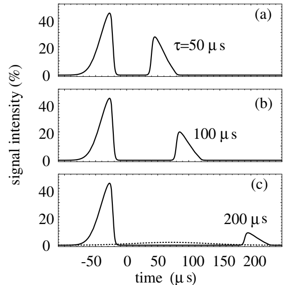
FIG. 3. Theoretical simulations of light storage in a three-state \Lambda system. Solid curves in each graph correspond to the experimental conditions of Figs. 2a–2c. Dephasing of the coherence is modeled by an exponential with a decay constant of 150 \mu\text{s} . The dotted line in Fig. 3c corresponds to the usual EIT propagation with a cw control field of 5 times weaker intensity than the input value of the dynamic case.
